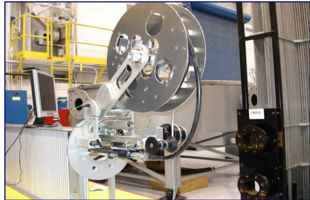
Ultra sludge lance system for tubesheet cleaning
